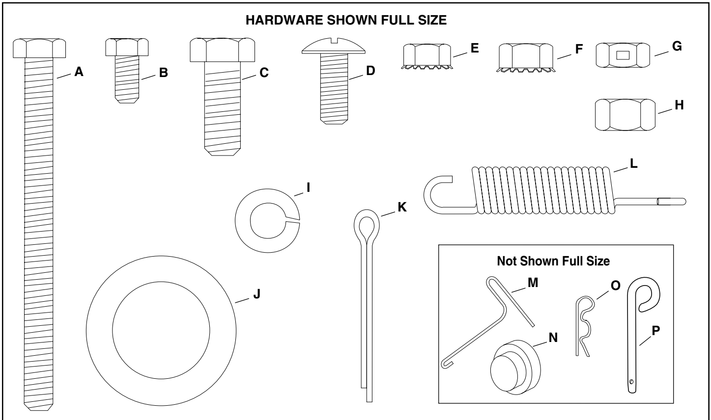
FIGURE 1 - HARDWARE PACK
